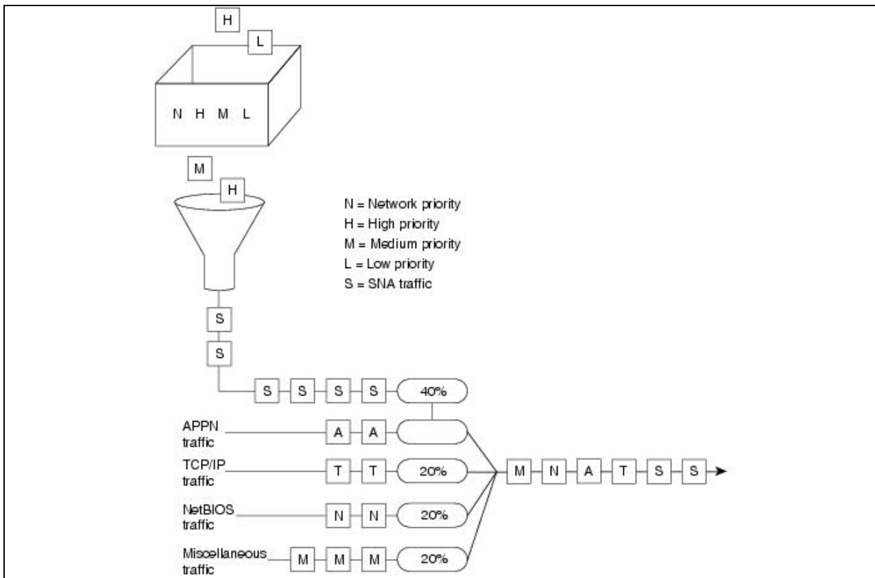
Figure: Custom queuing
