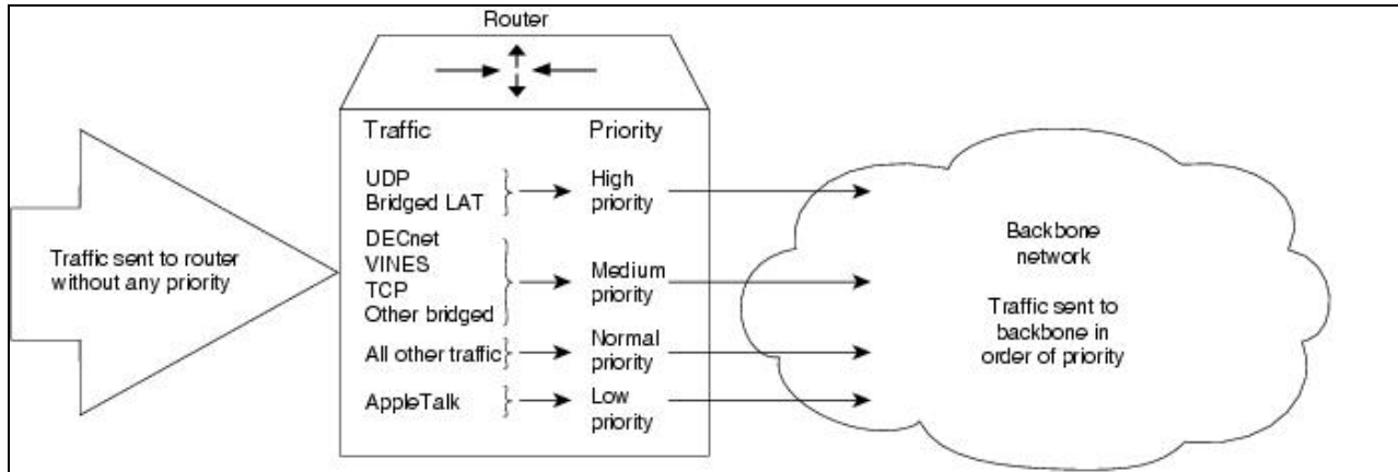
Figure: Priority queuing
