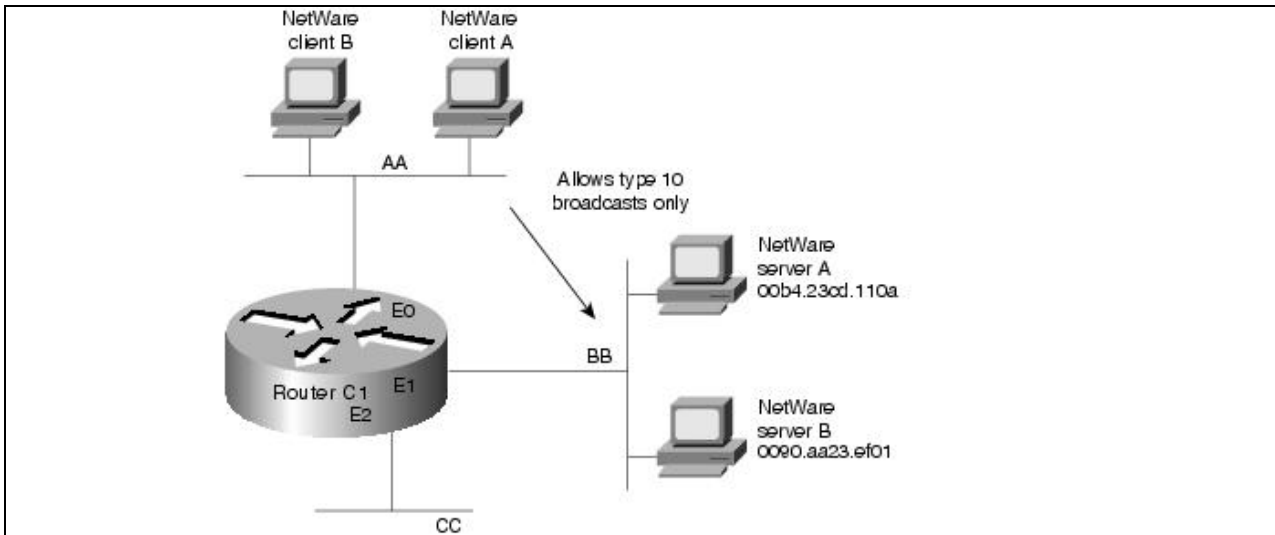
Figure: Sample network map illustrating helper address broadcast control
