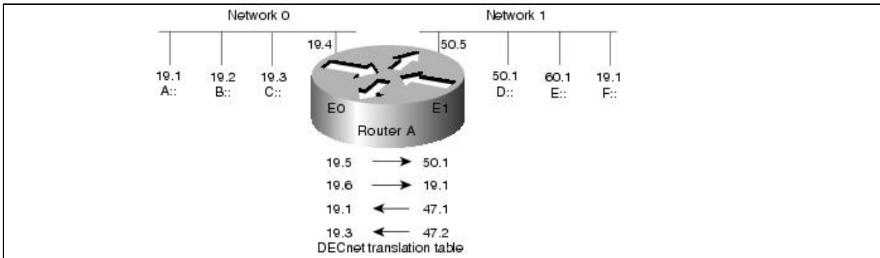
Figure: Sample DECnet ATG implementation
