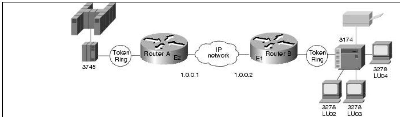
Figure: LU prioritization implementation
