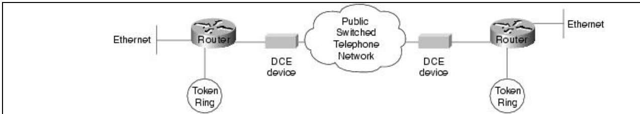
Figure: The Dial-on-demand routing environment
