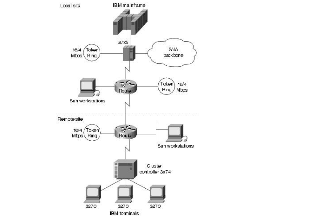
Figure: STUN configuration
