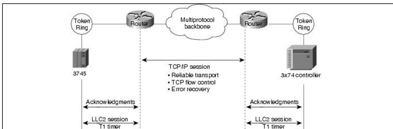
Figure: Local session termination over multiprotocol backbone
