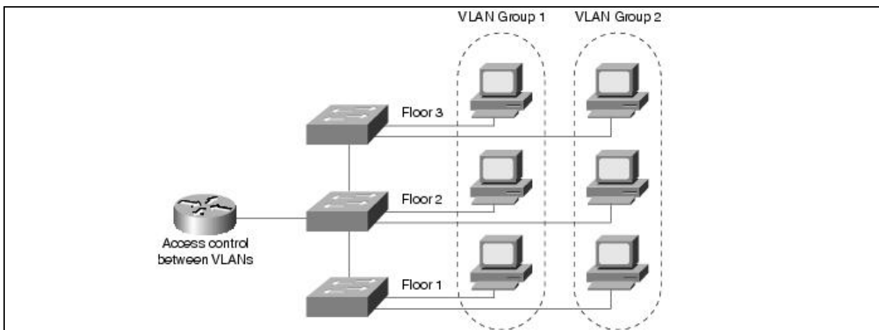
Figure: Role of switches and routers in VLANs
