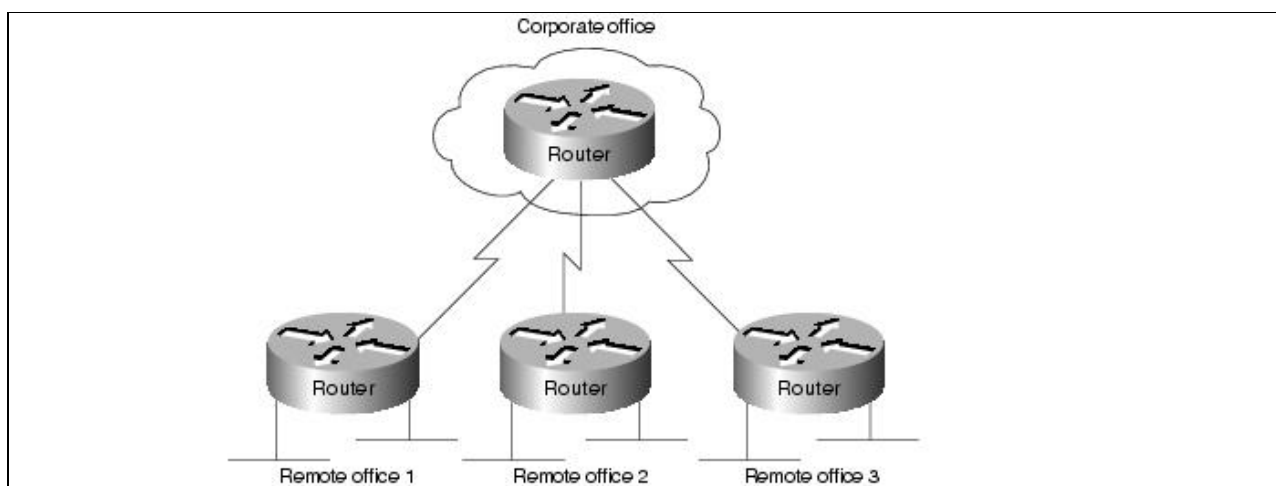
Figure: Typical nonredundant internetwork design
