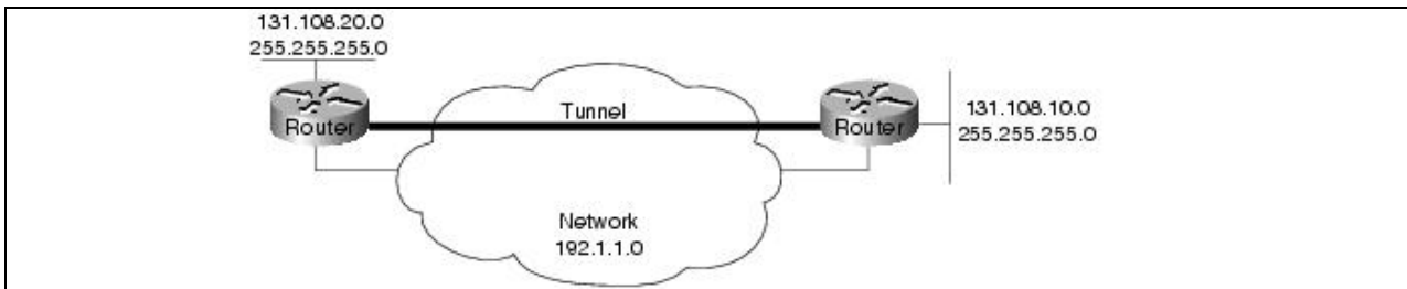
Figure: Connecting discontinuous networks with tunnels
