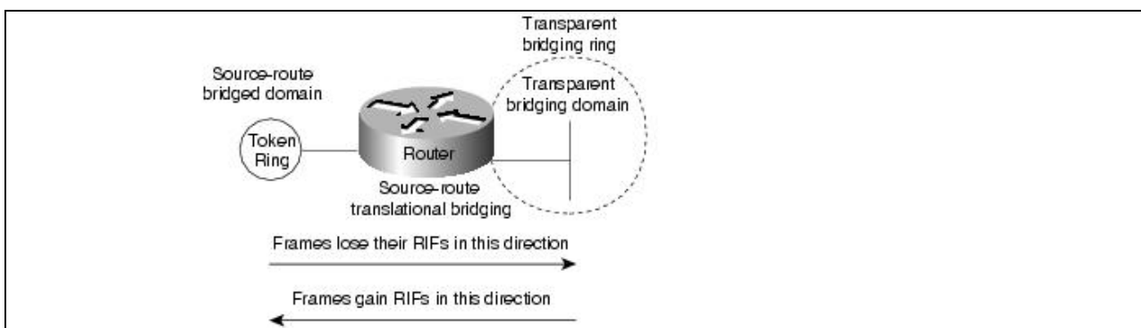
Figure: Source-route translational bridging topology
