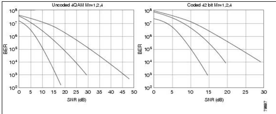
Figure: BER Against Signal-to-Noise for Coded and Uncoded Data Streams
