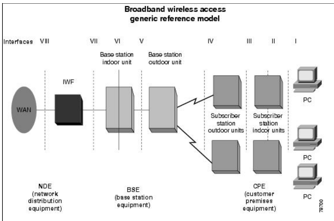
Figure: Generic Reference Model for Broadband Wireless Access
