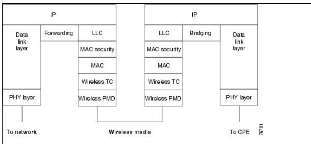
Figure: Wireless Protocol Stack for Network Management and Operation
