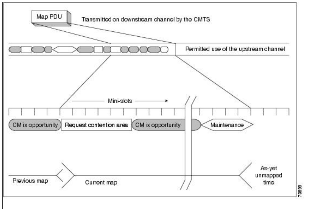
Figure: Frame Allocation MAP
