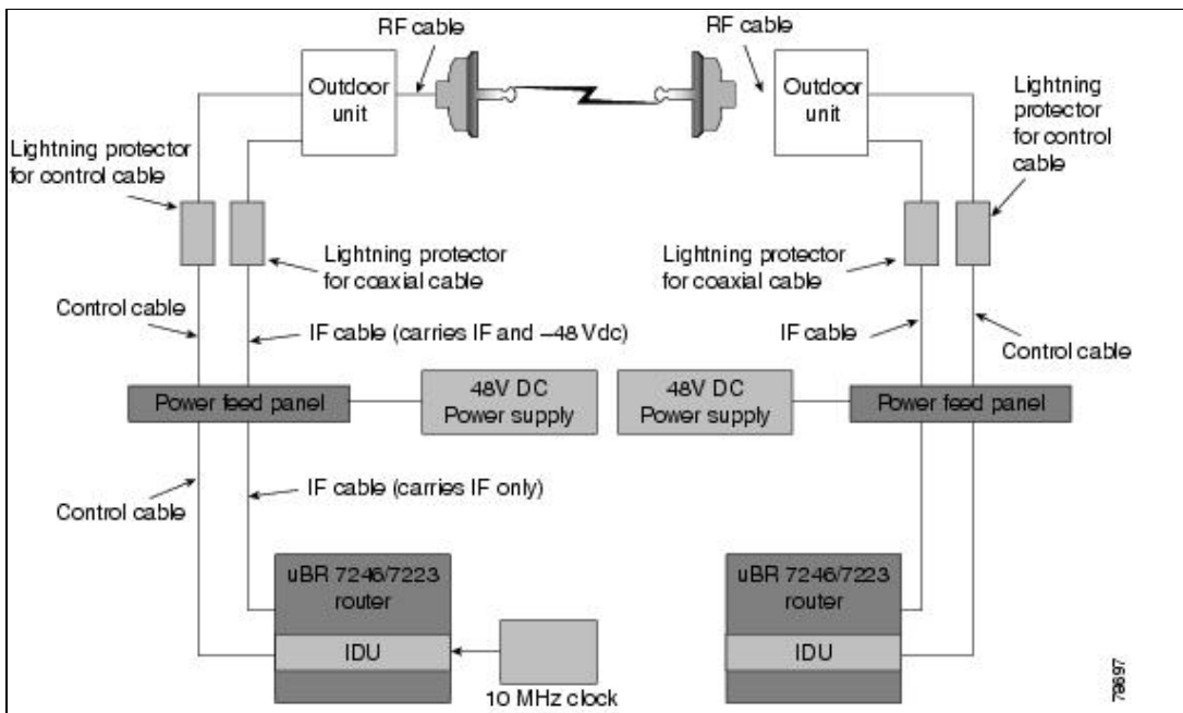
Figure: Open Standard Wireless Architecture
