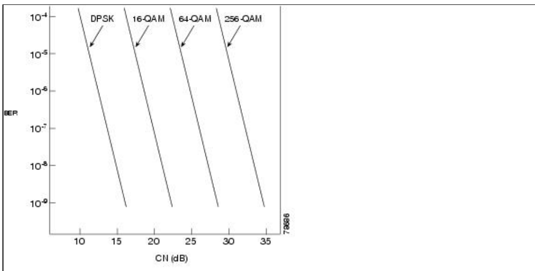
Figure: Error Rates for PSK and QAM Systems
