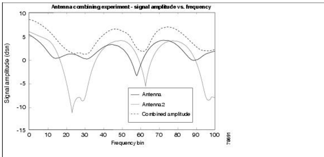
Figure: Multipath Reception
