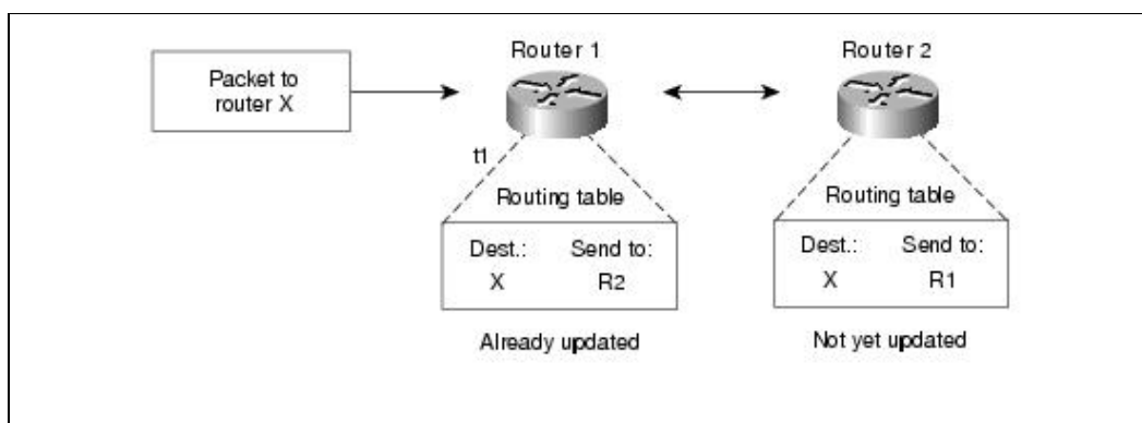
Figure: Destination/Next Hop Associations Determine the Data's Optimal Path
