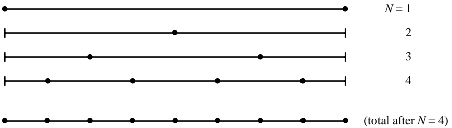
Figure 4.2.1. Sequential calls to the routine trapszd incorporate the information from previous calls and evaluate the integrand only at those new points necessary to refine the grid. The bottom line shows the totality of function evaluations after the fourth call. The routine qsimp , by weighting the intermediate results, transforms the trapezoid rule into Simpson's rule with essentially no additional overhead.
