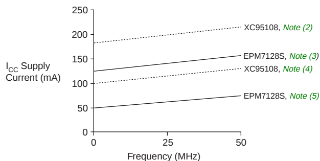
Figure 2. MAX 7000S & XC9500 Power Consumption Note (1)
