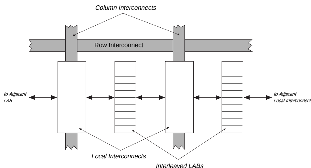
Figure 1. Interleaved LAB Feature of the FLEX 6000 Architecture
