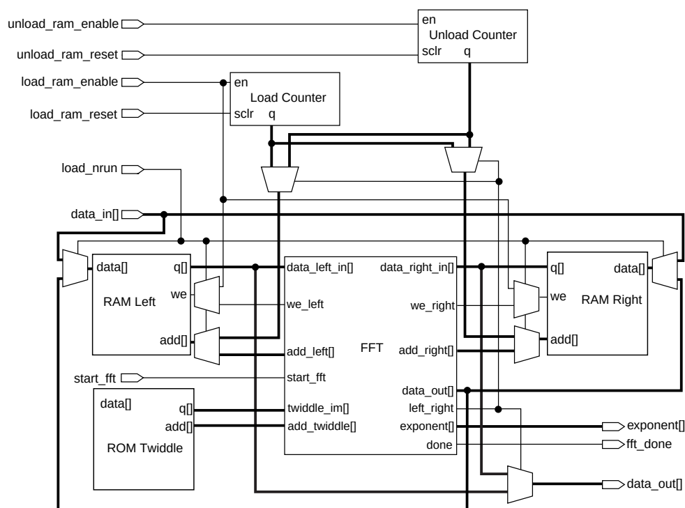
Figure 1. Block Diagram of an FFT Function
