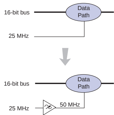
Figure 2. ClockBoost Circuitry
