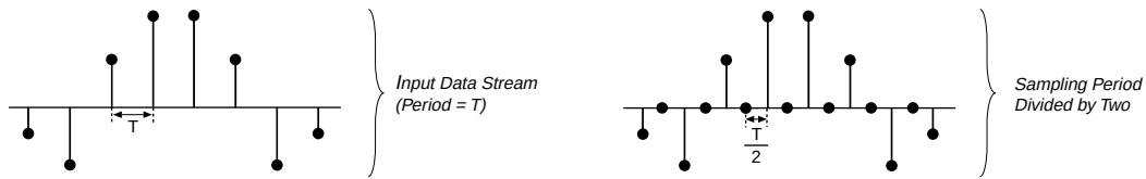
Figure 3. Stuffing Zeros into the Data Stream
