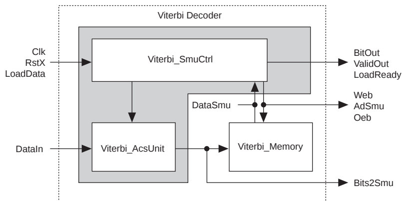
Figure 2. Viterbi Decoder Block Diagram
