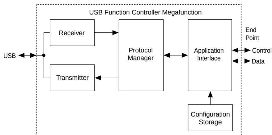
Figure 1. USB Function Controller Megafunction Block Diagram
