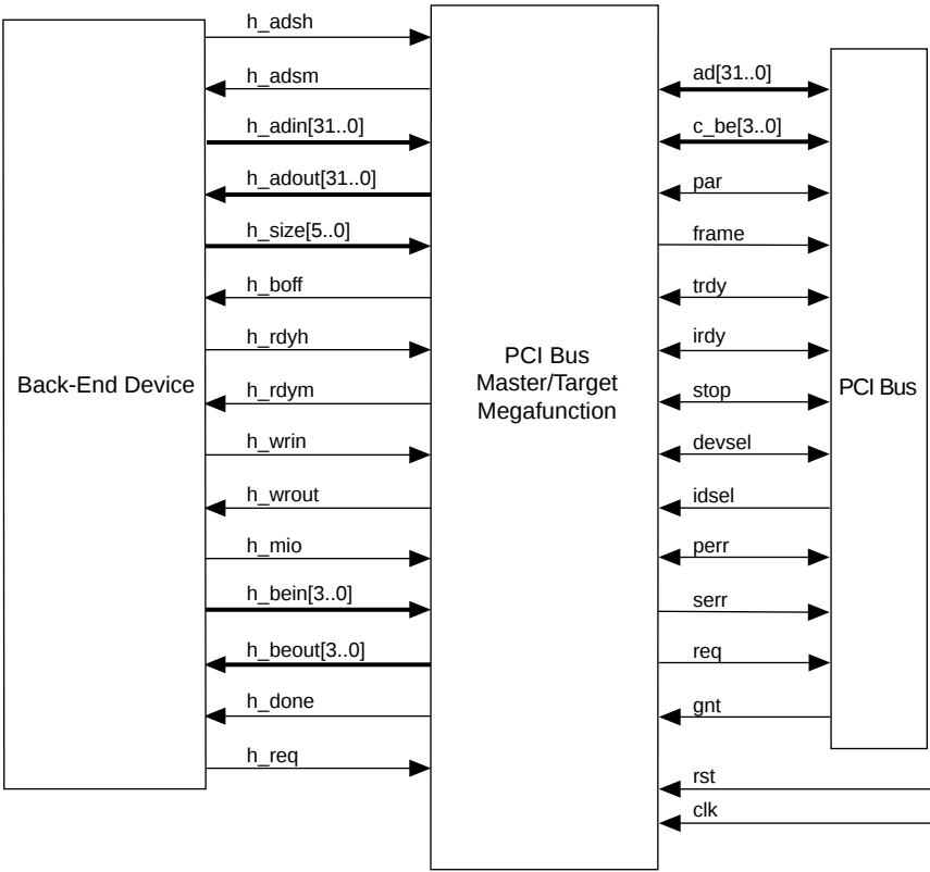
Figure 2. Signals for the EC210 PCI Bus Master/Target Megafunction
