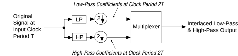
Figure 2. FASTMAN Biorthogonal Wavelet Filter Megafunction
