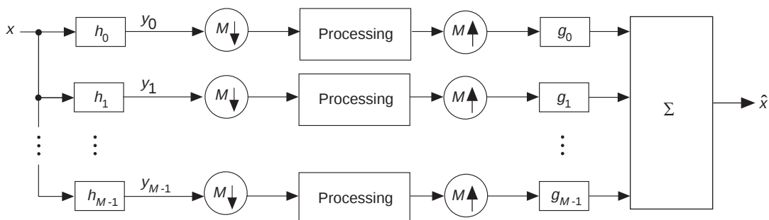
Figure 1. Incoming Signal Processed through a Filter Bank
