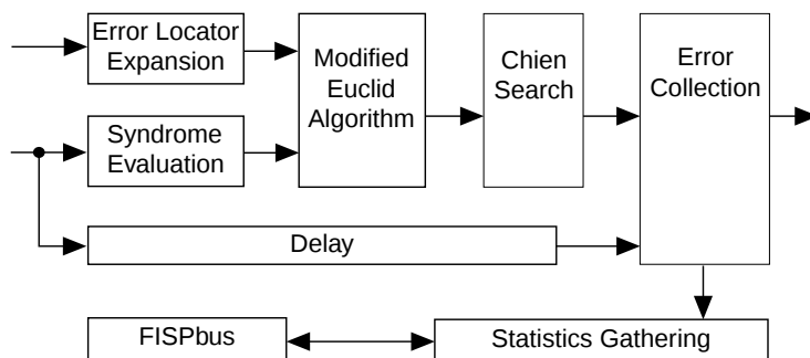
Figure 2. Reed-Solomon Decoder
