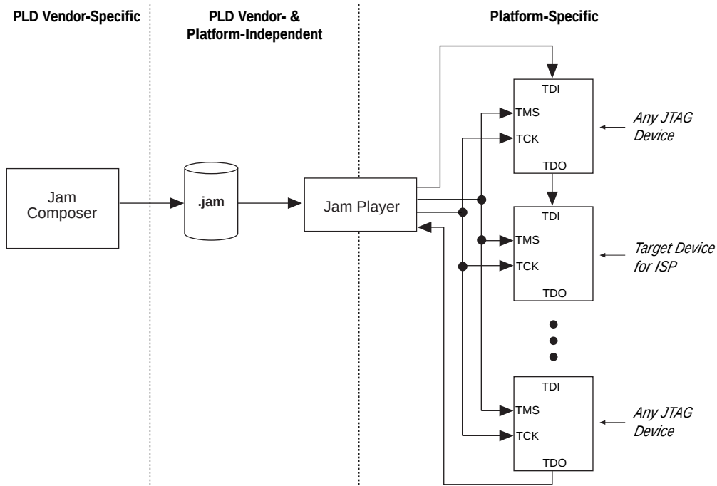
Figure 1. Basic Jam Flow
