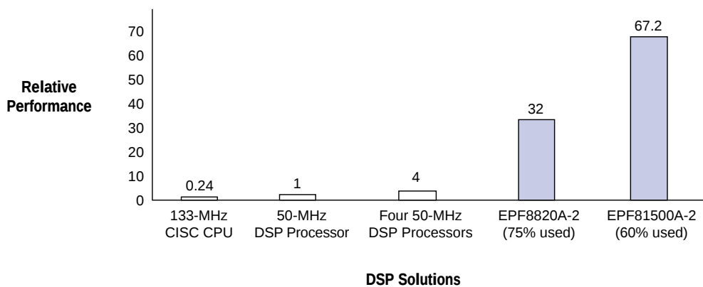
Figure 2. Performance Comparison for 16-Tap, 8-Bit FIR Filter
