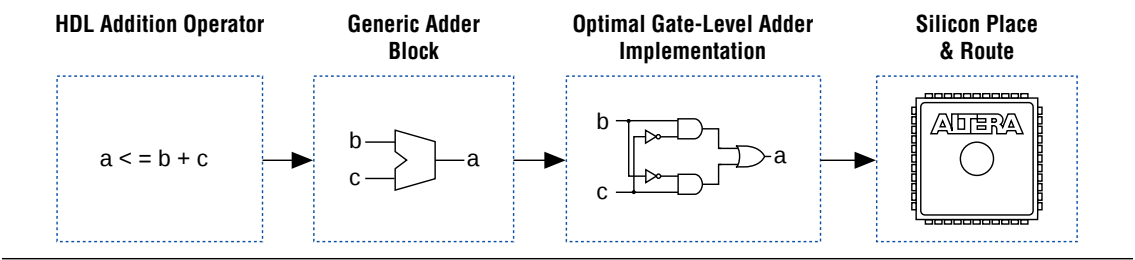
Figure 1. Inference Process
