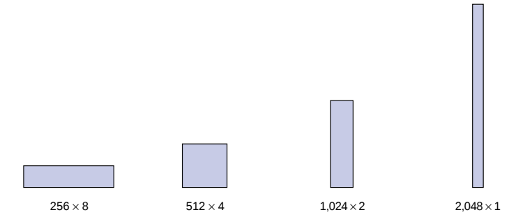
Figure 2. EAB Memory Configurations
