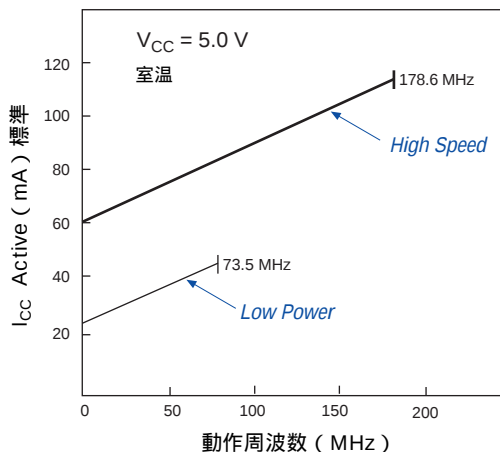
EPM7064S
