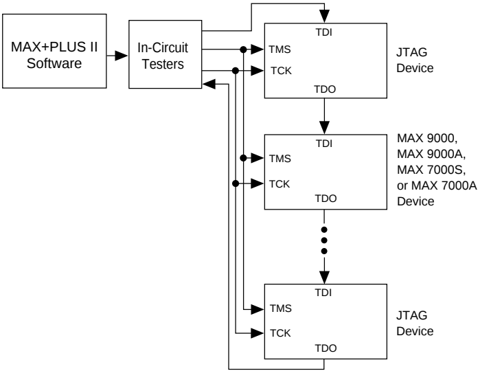
Figure 5. Programming Flow between Altera & JTAG Technologies
