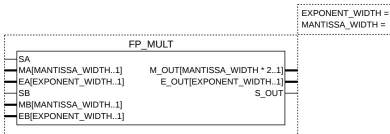
Figure 1. fp_mult Symbol
