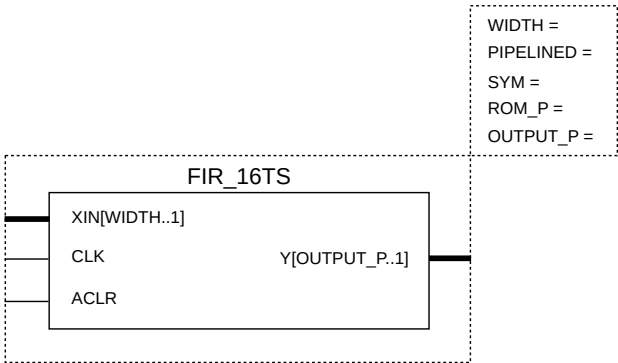
Figure 10. Serial FIR Filter Symbol
