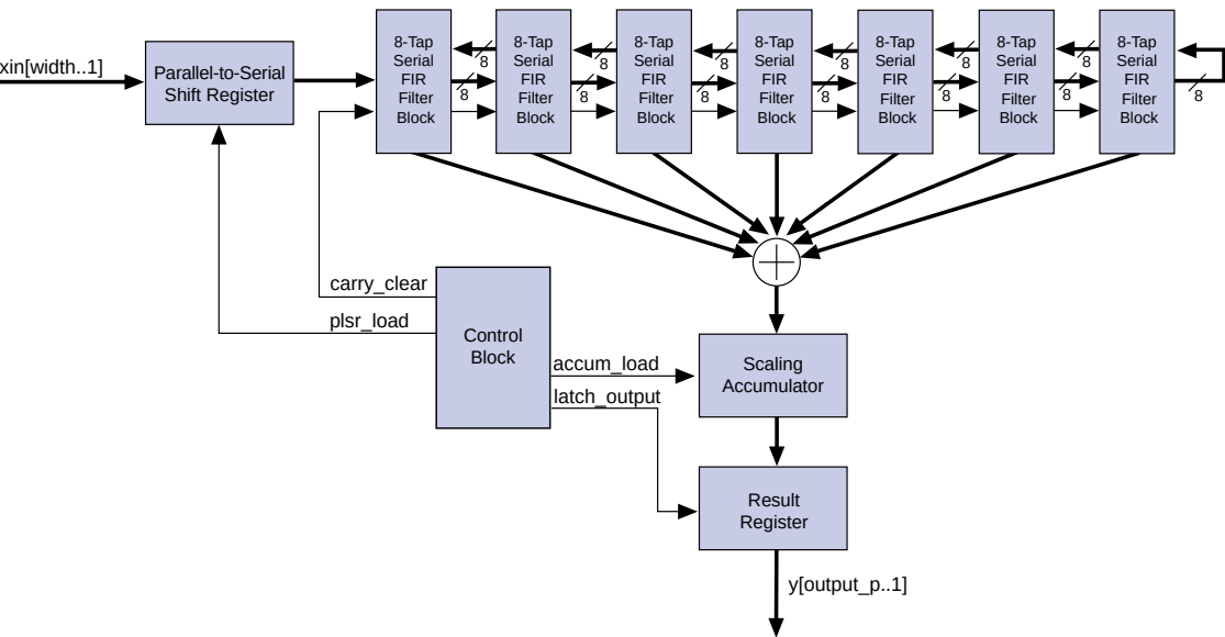
Figure 12. FIR_64TS Filter Block Diagram
