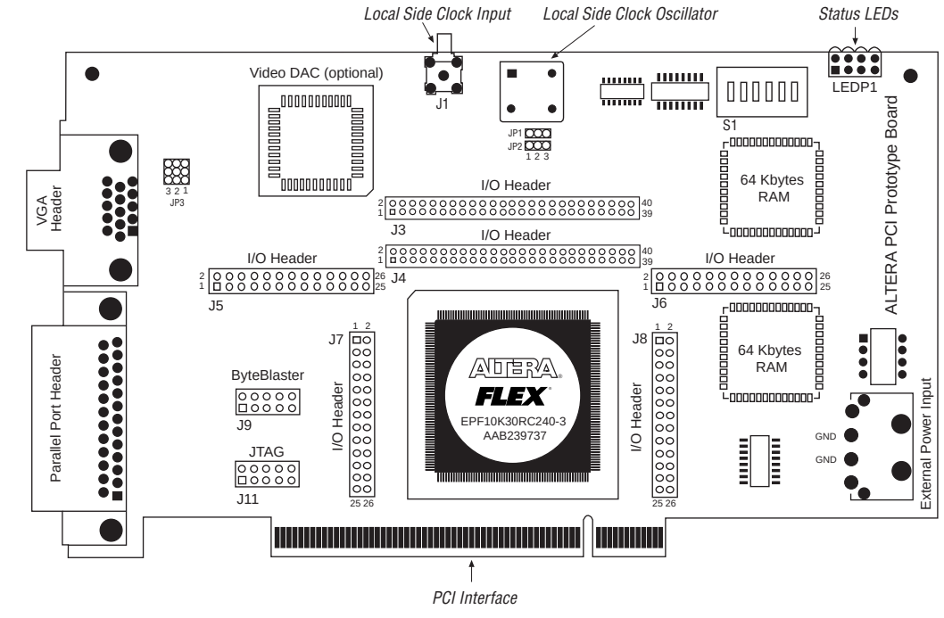
Figure 1. PCI Prototype Board Block Diagram
