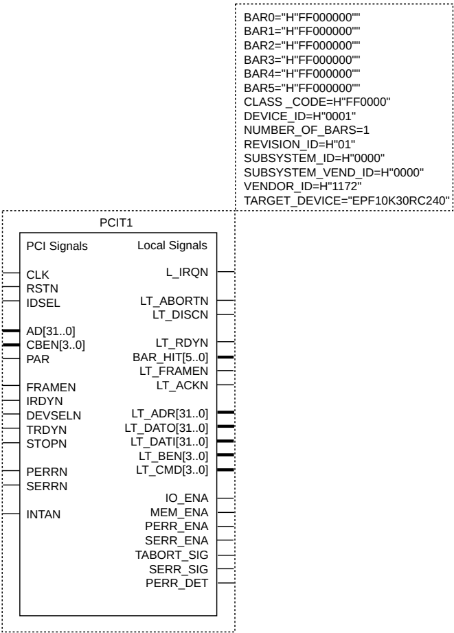
Figure 1. pcit1 Symbol
