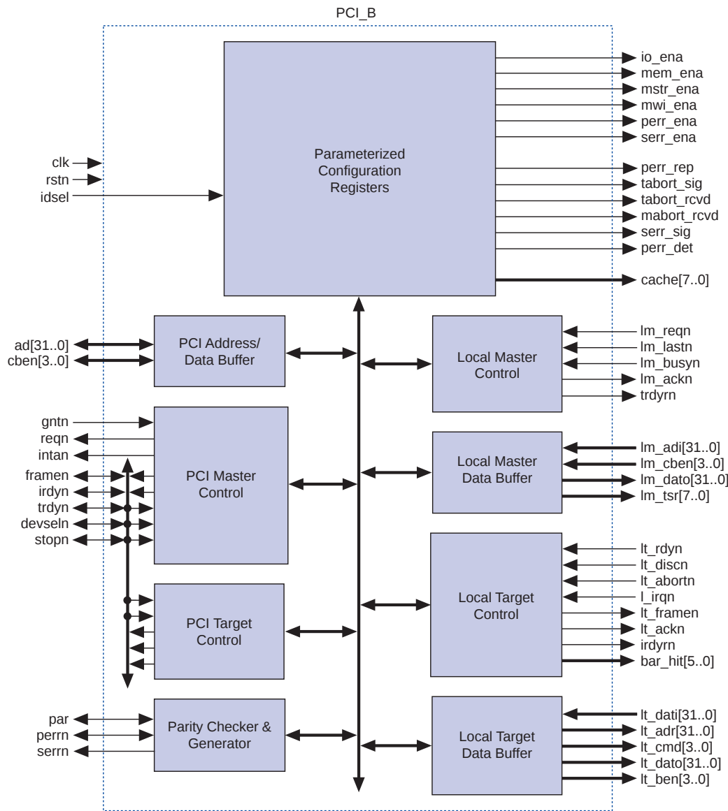
Figure 2. pci_b Functional Block Diagram
