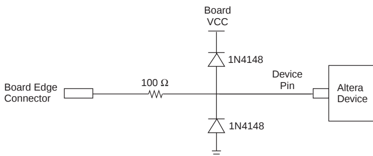
Figure 2. Hot-Socket Protection
