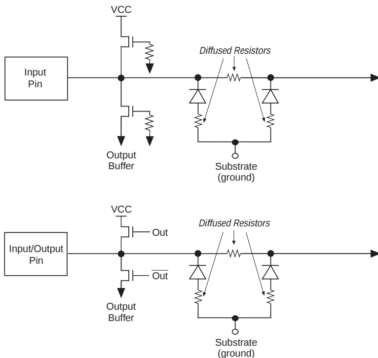
Figure 3. Altera Device Input Protection Structures
