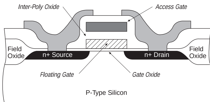
Figure 4. EPROM Cell Construction
