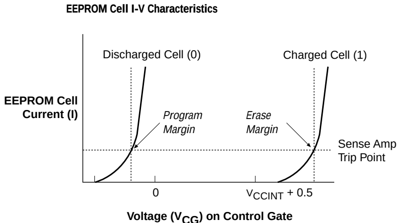
Figure 2. Current vs. Voltage Relationships of EEPROM Cells
