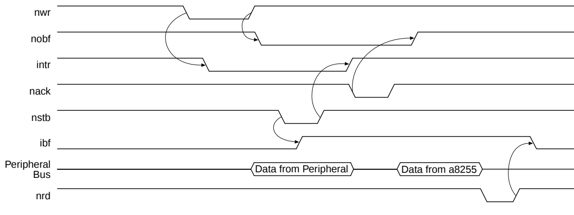
Figure 4. a8255 Mode 2 Functional Timing Waveforms
