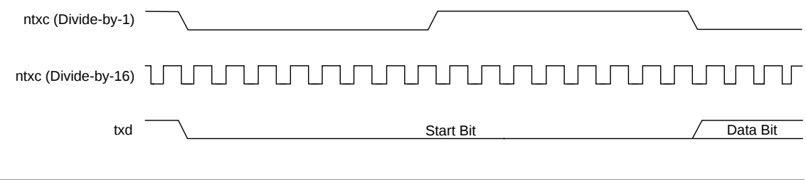
Figure 6. Transmitter Data & Clock Signals
