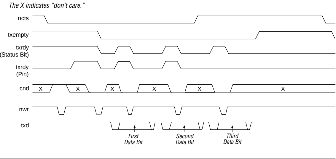
Figure 5. Transmitter Control & Error Signals (Asynchronous)
