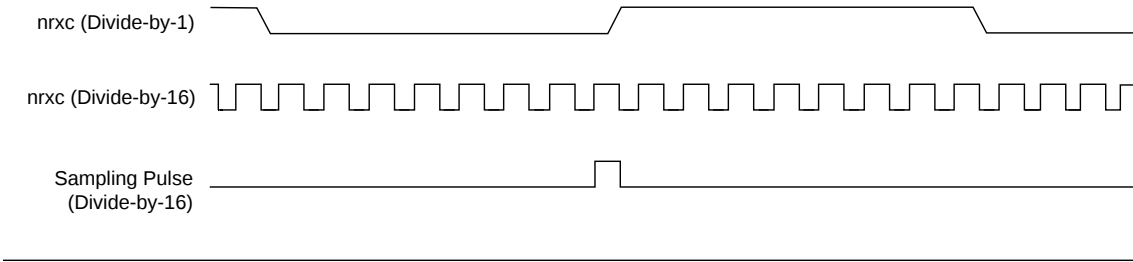
Figure 3. Receiver Clock Signals
