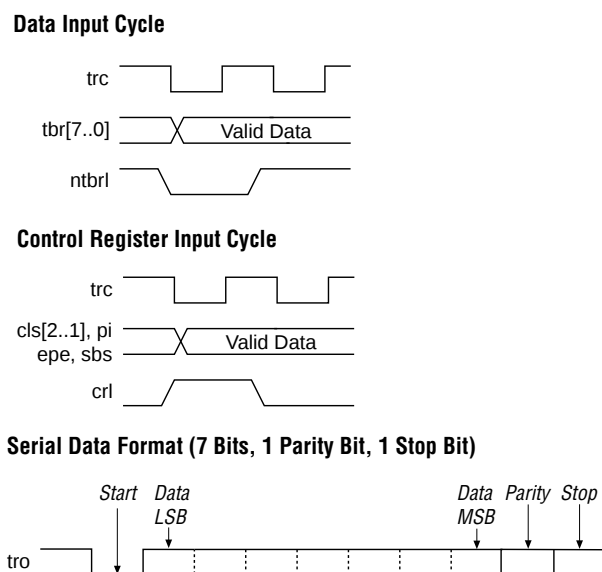
Figure 3. a6402 Functional Timing Waveforms
