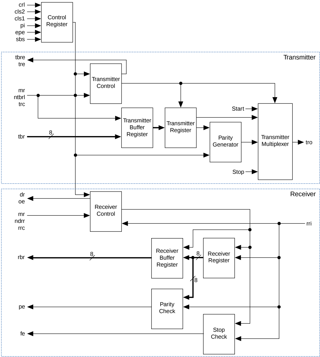
Figure 2. a6402 Block Diagram
