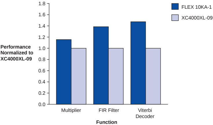
Figure 4. Normalized Common Megafunction Results
