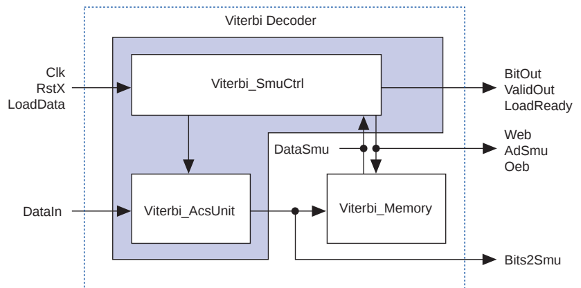
Figure 3. Viterbi Decoder Megafunction Block Diagram
