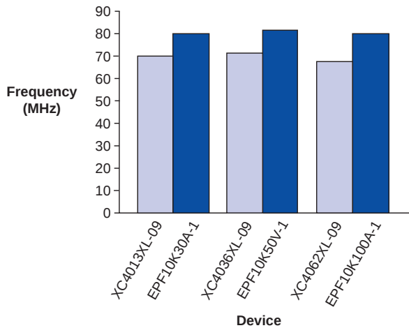
Figure 1. Multiplier Performance Results
