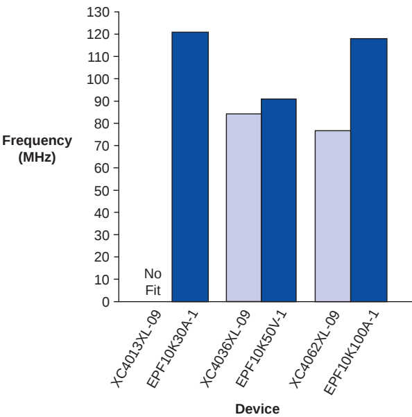
Figure 2. FIR Filter Performance Results
