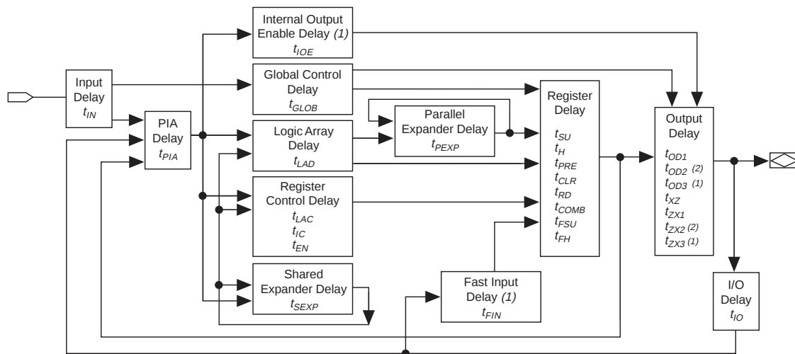
Figure 1. MAX 7000 Device Timing Model
