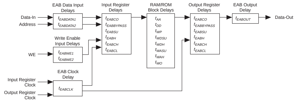
Figure 8. FLEX 10K Device EAB Timing Model
