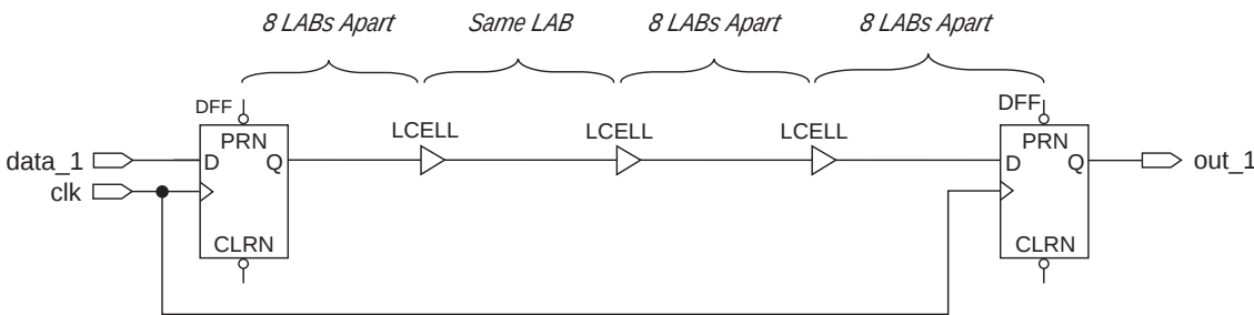
Figure 2. t DDR Circuit Path for 36-Column FLEX 10K Devices
