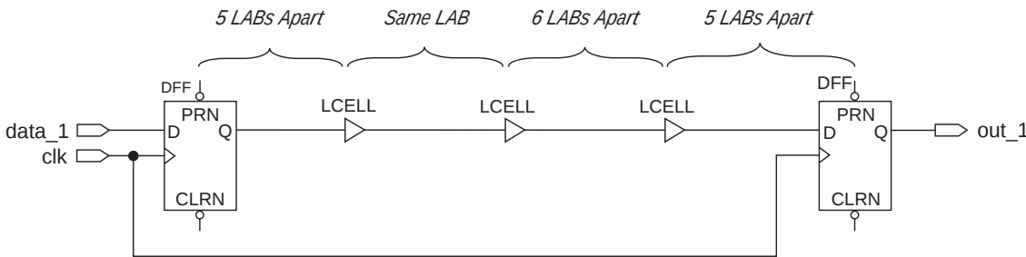
Figure 1. t DDR Circuit Path for 24-Column FLEX 10K Devices
