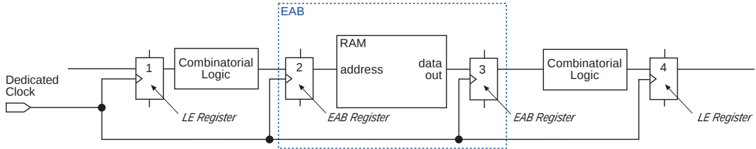
Figure 11. EAB Timing Delays
