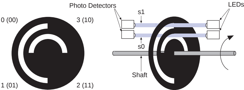
Figure 11. Shaft Encoder for 2-Bit Gray Code
