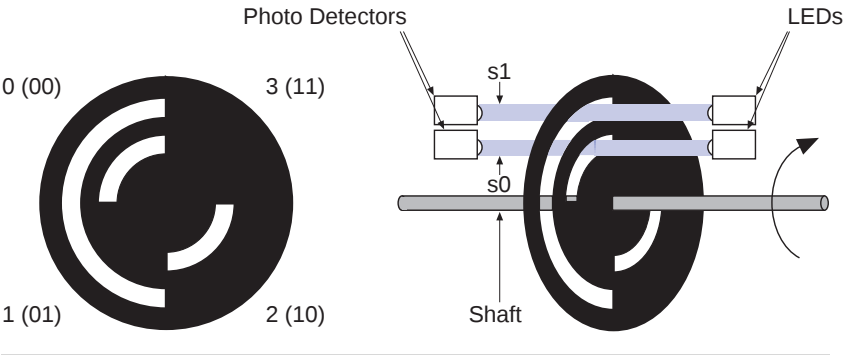
Figure 8. Straight Binary Shaft Encoder
