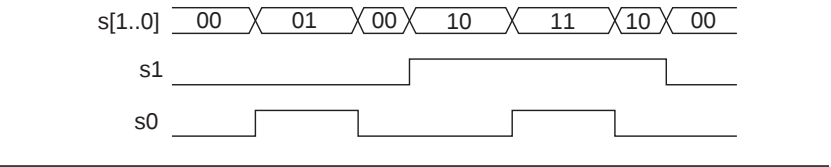
Figure 10. Waveforms Caused by Misaligned Sensors
