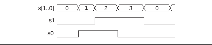
Figure 12. Gray Code Sequence with Significant Misalignment
