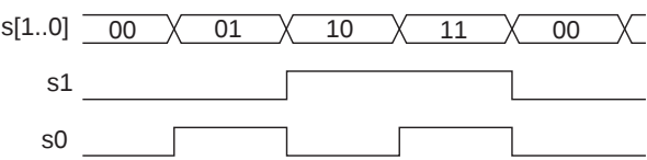
Figure 9. Ideal Waveforms of s1 & s0
