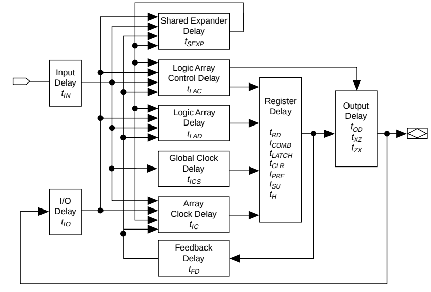
Figure 1. Single-LAB MAX 5000 Device Timing Model
