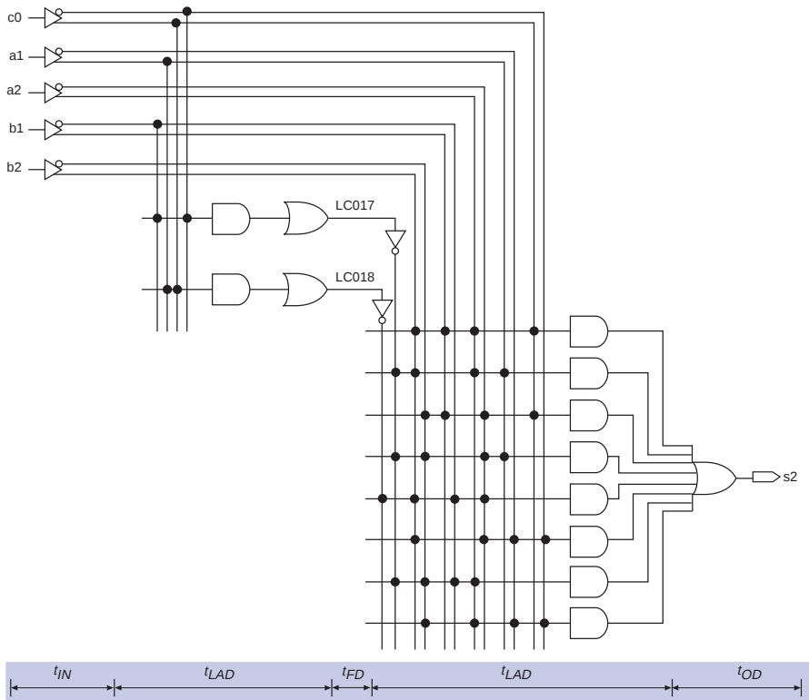
Figure 8. Adder Equations Mapped to Classic Architecture
