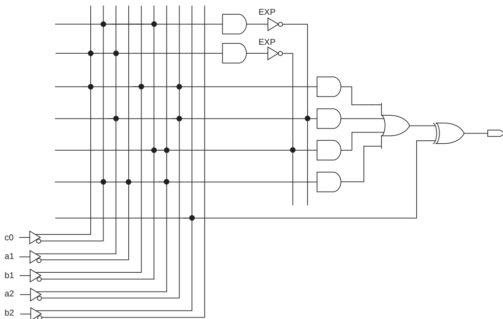
Figure 7. Adder Equations Mapped to MAX 9000 Architecture
