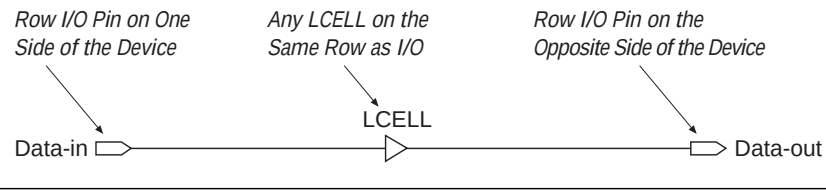
Figure 1. Test Circuit for t_{PD1}
