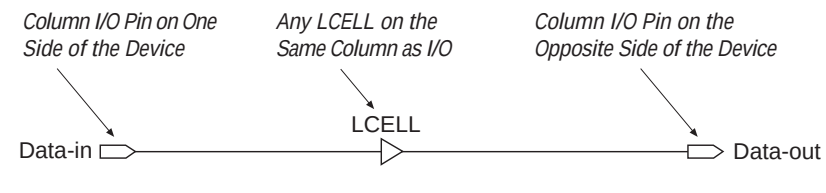
Figure 2. Test Circuit for t_{PD2}
