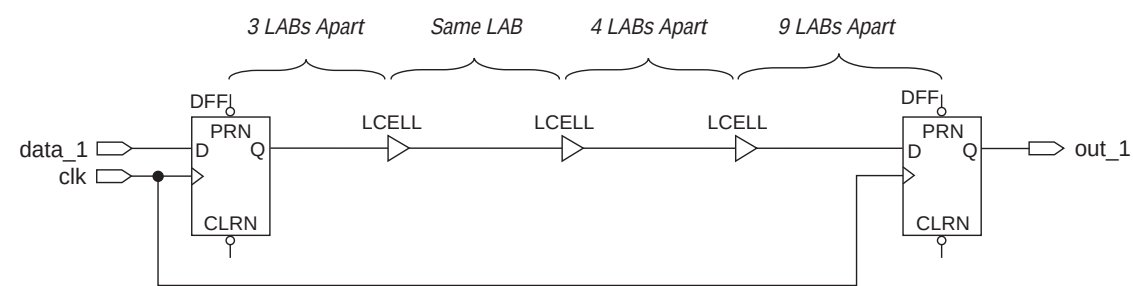
Figure 1. Path for t DDR Circuit for 21-Column FLEX 8000 Devices
