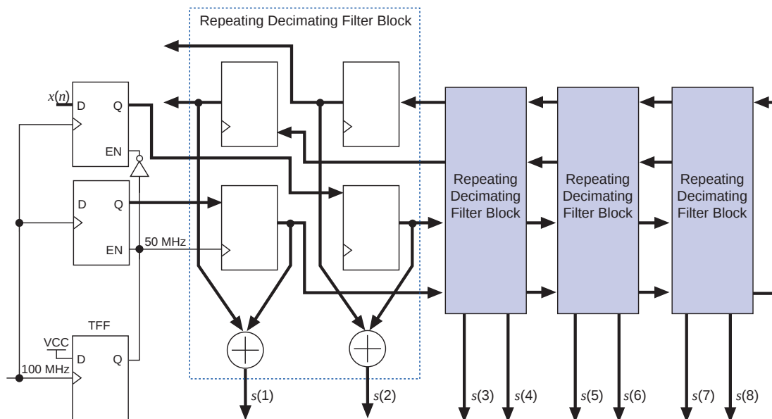
Figure 15. FLEX Decimating Filter
