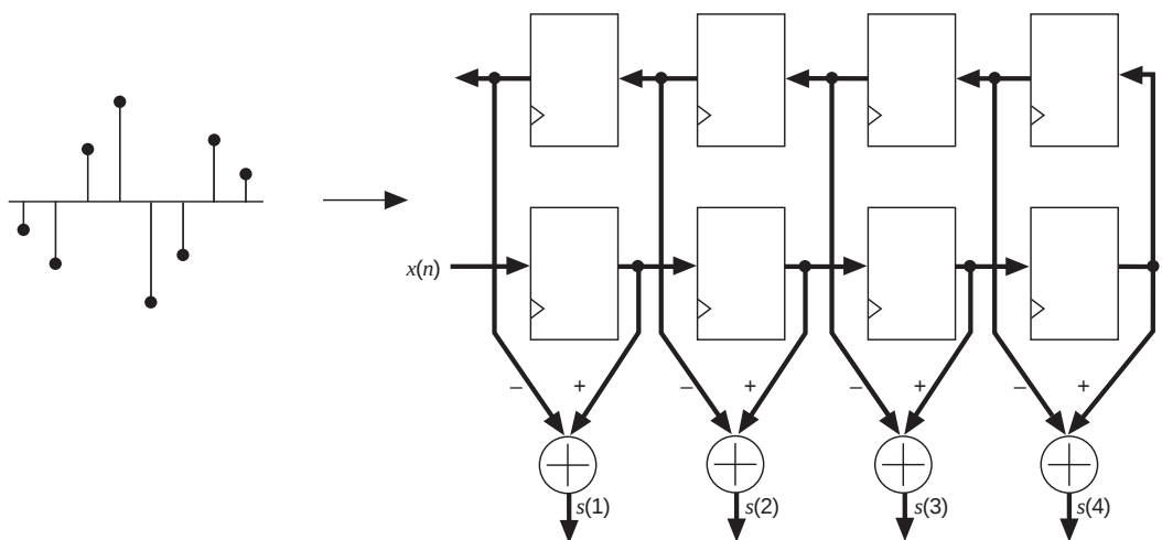
Antisymmetric Impulse Response
