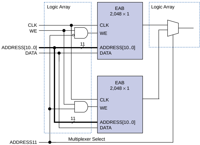
Figure 4. Multiplexed EABs
