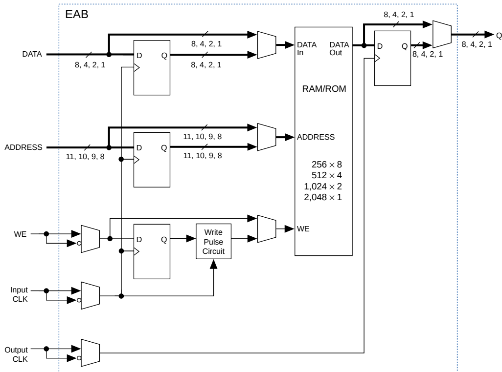
Figure 1. EAB Block Diagram
