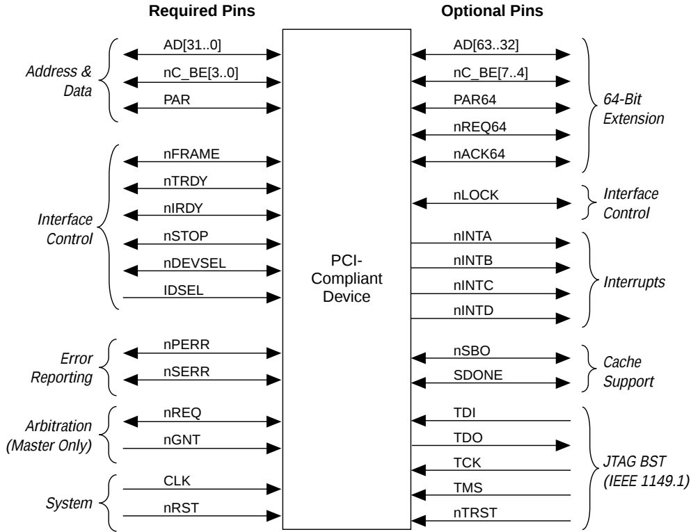
Figure 2. Required & Optional Pins
