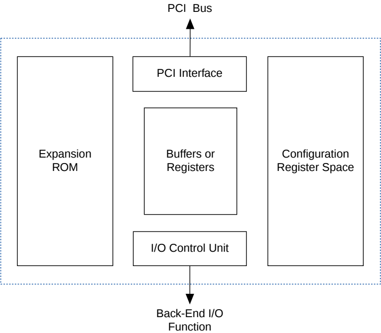
Figure 3. Generic PCI Controller Architecture
